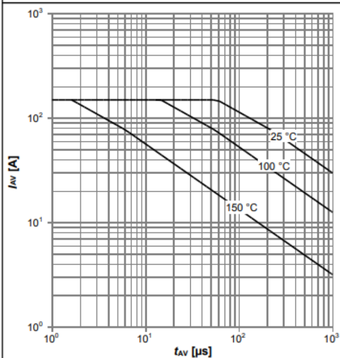
Diagram 13: Avalanche characteristics
