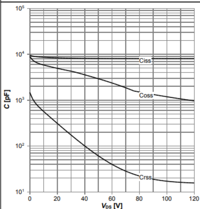
Diagram 11: Typ. capacitances
