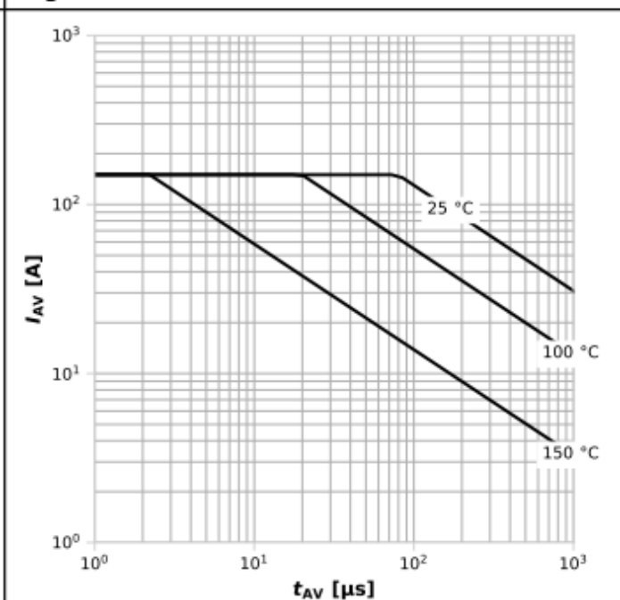
Diagram 14: Avalanche characteristics
