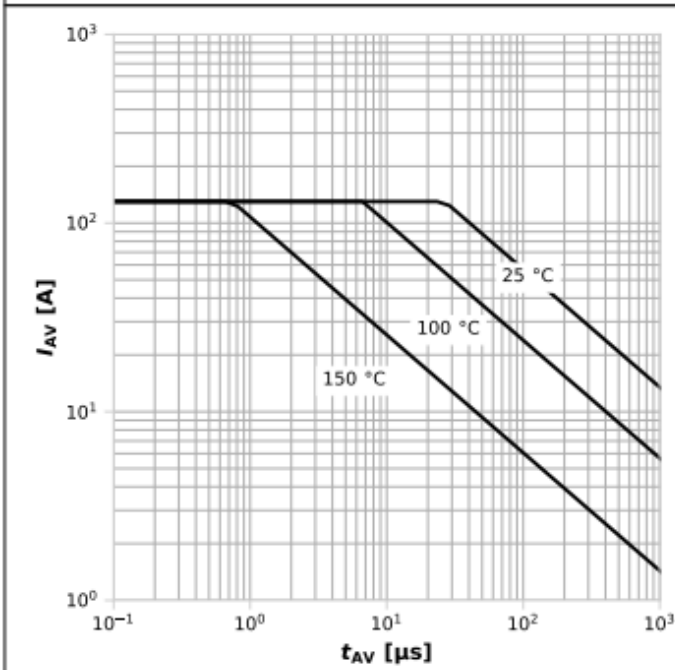
Diagram 13: Avalanche characteristics
