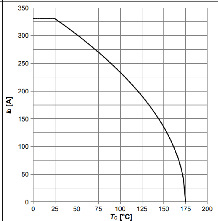
Diagram 2: Drain current
