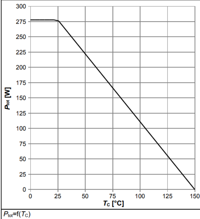
Diagram 1: Power dissipation
