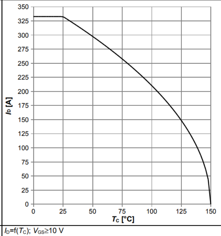
Diagram 2: Drain current
