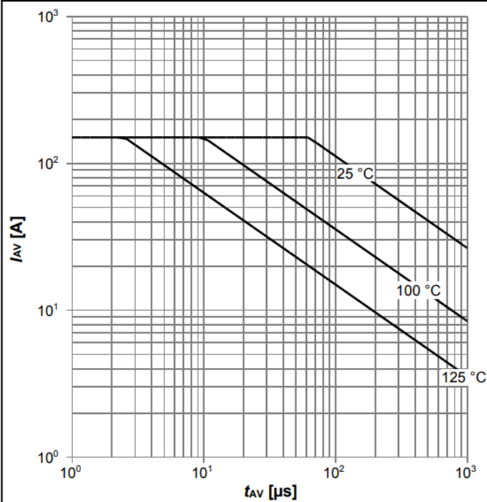
Diagram 13: Avalanche characteristics
