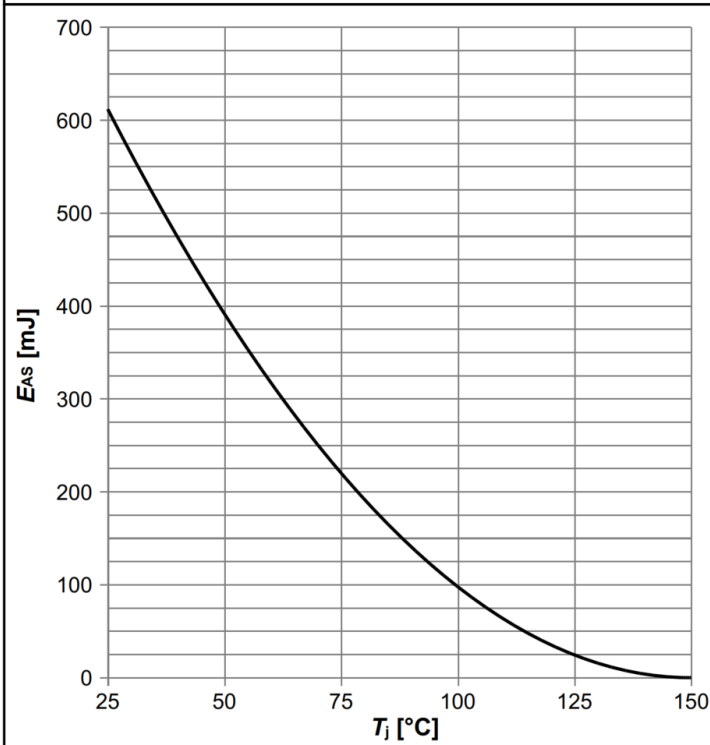
Diagram 13: Avalanche energy
