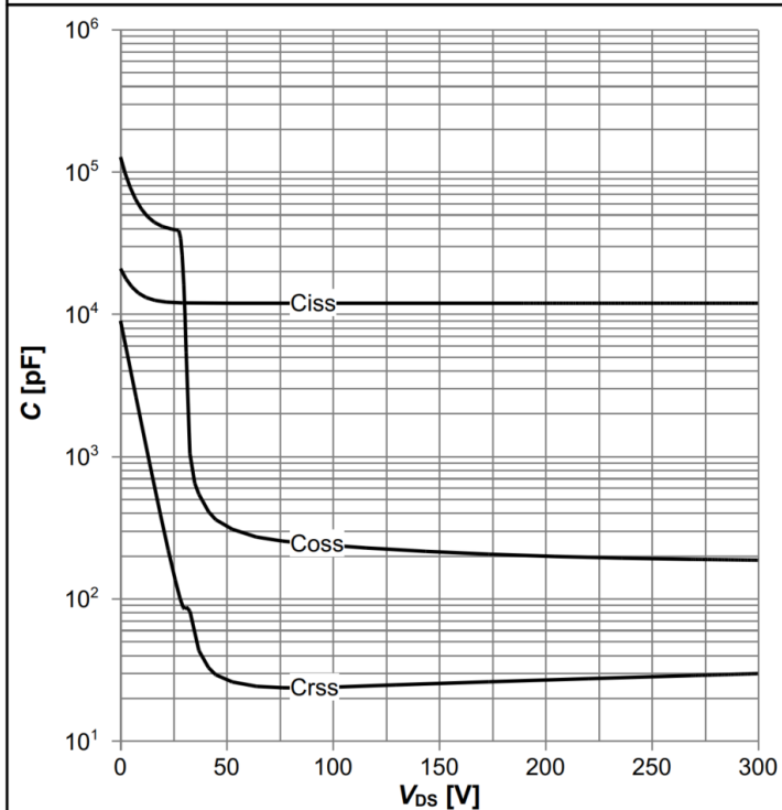
Diagram 15: Typ. capacitances
