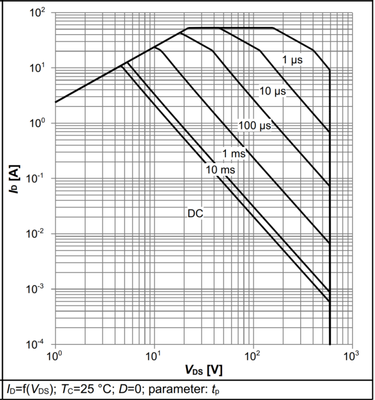
Diagram 2: Safe operating area
