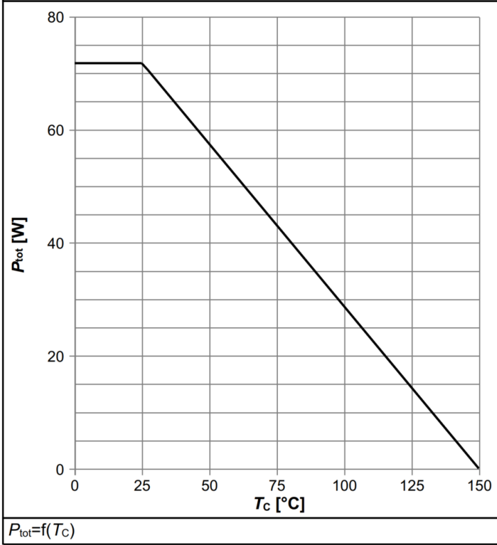
Diagram 1: Power dissipation
