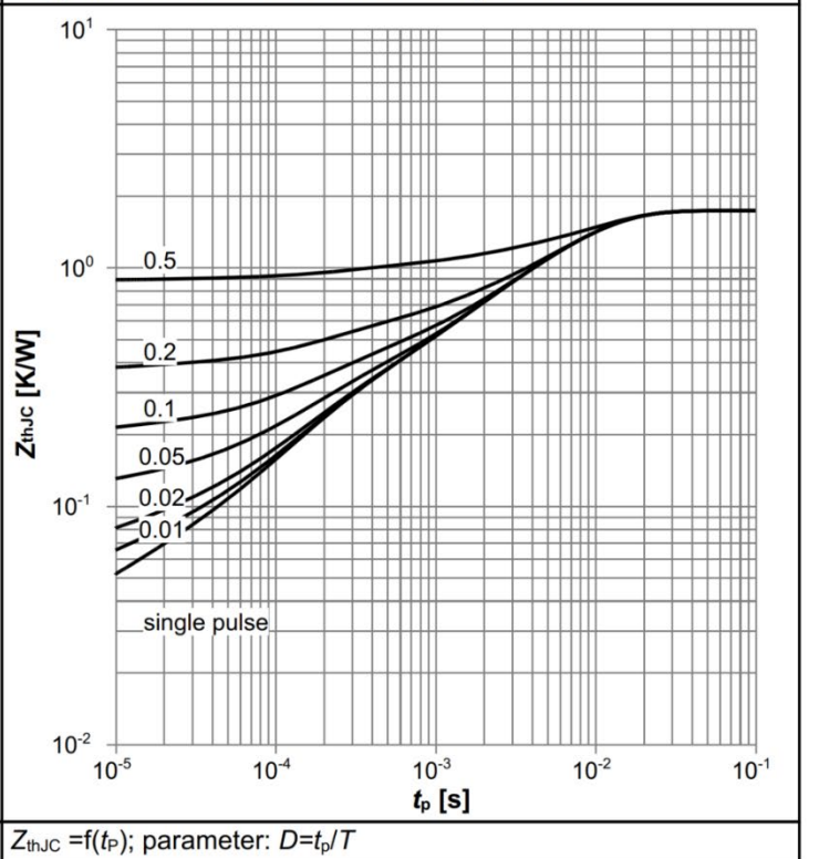
Diagram 4: Max. transient thermal impedance
