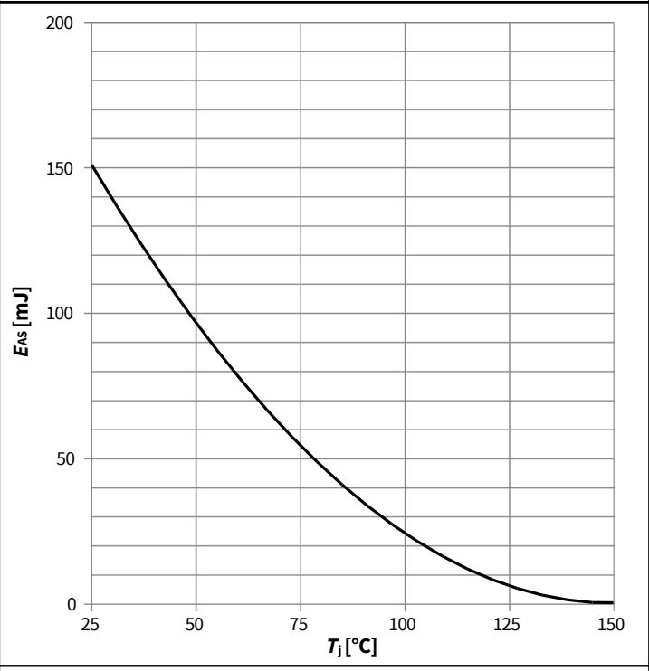
Diagram 12: Avalanche energy
