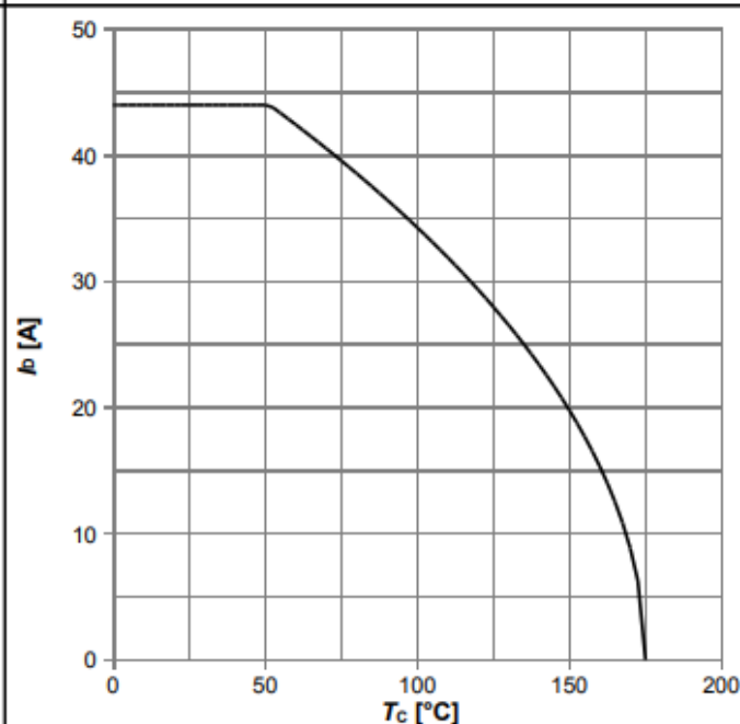
Diagram 2: Drain current
