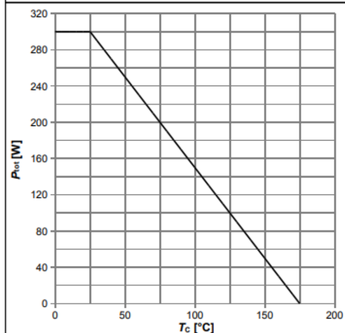
Diagram 1: Power dissipation
