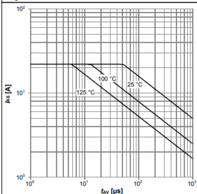
Diagram 13: Avalanche characteristics
