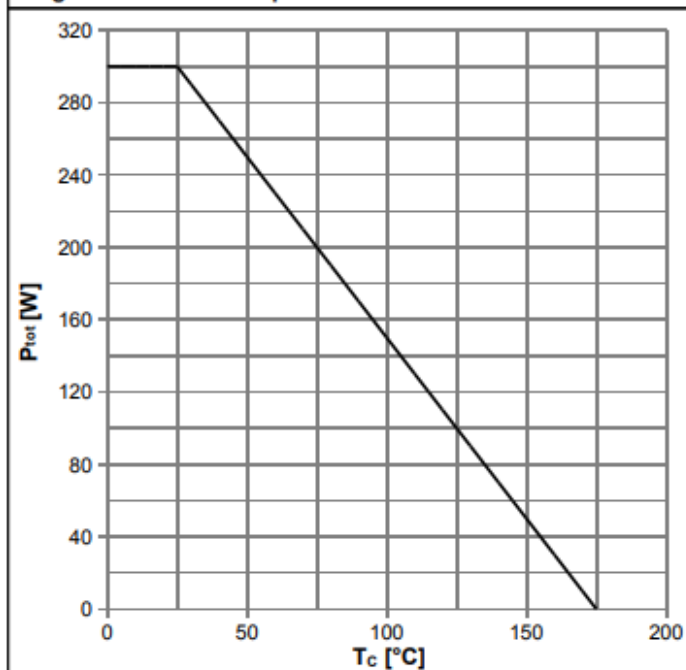
Diagram 1: Power dissipation
