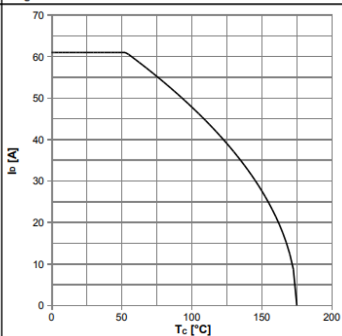
Diagram 2: Drain current
