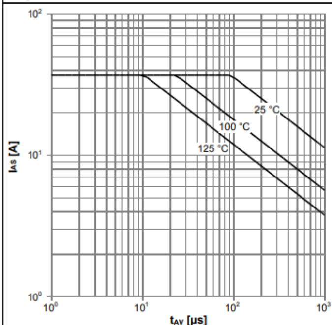
Diagram 13: Avalanche characteristics
