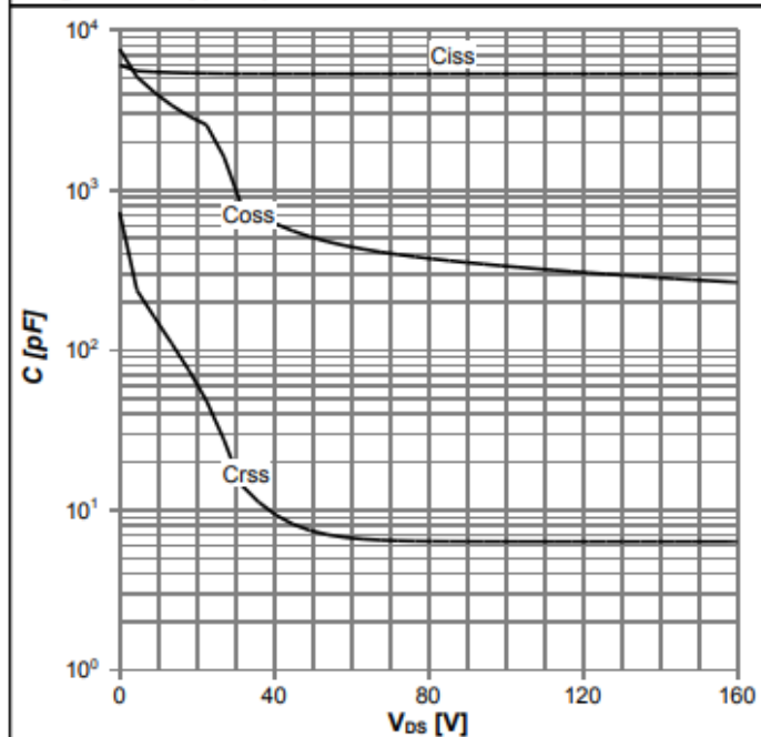
Diagram 11: Typ. capacitances
