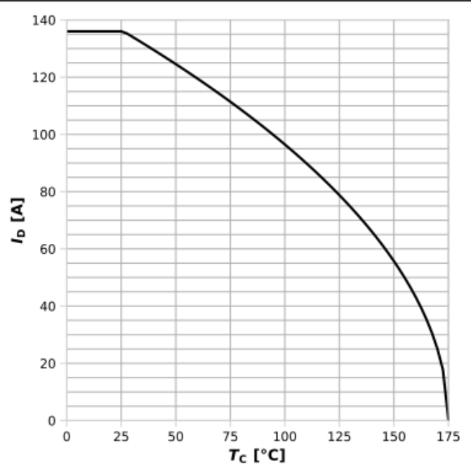
Diagram 2: Drain current
