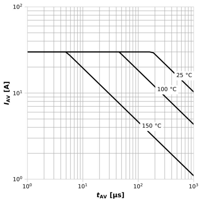
Diagram 13: Avalanche characteristics
