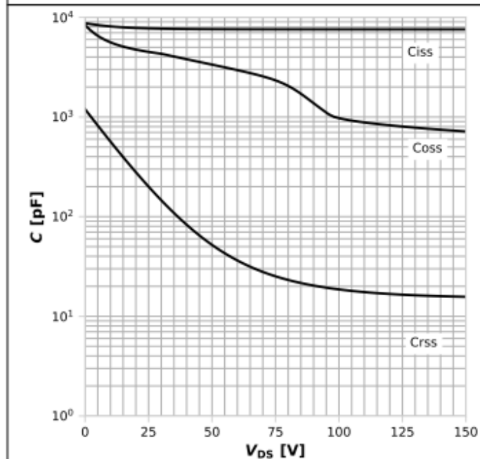
Diagram 11: Typ. capacitances
