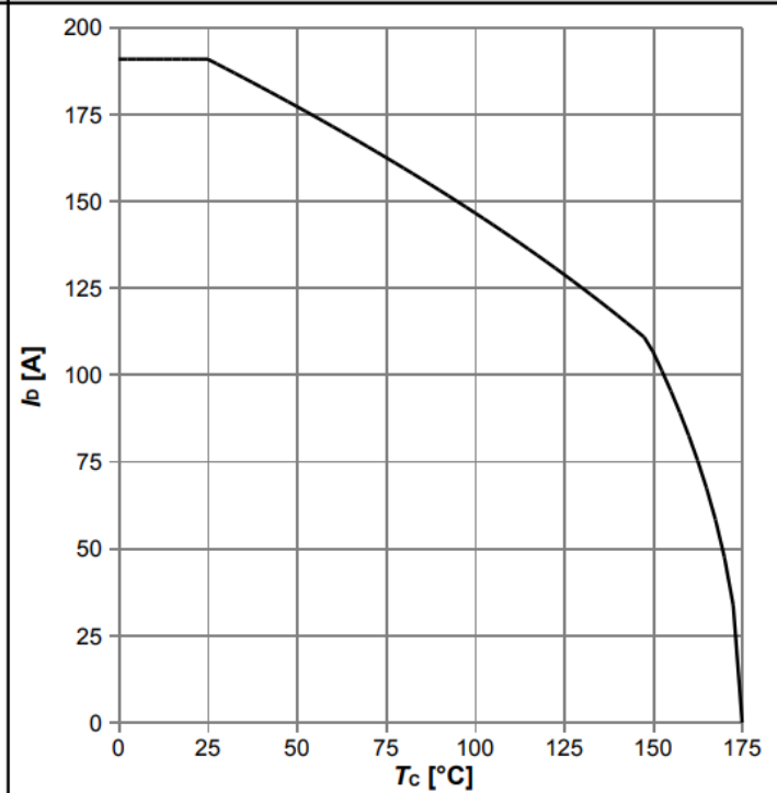
Diagram 2: Drain current
