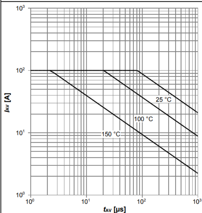
Diagram 13: Avalanche characteristics
