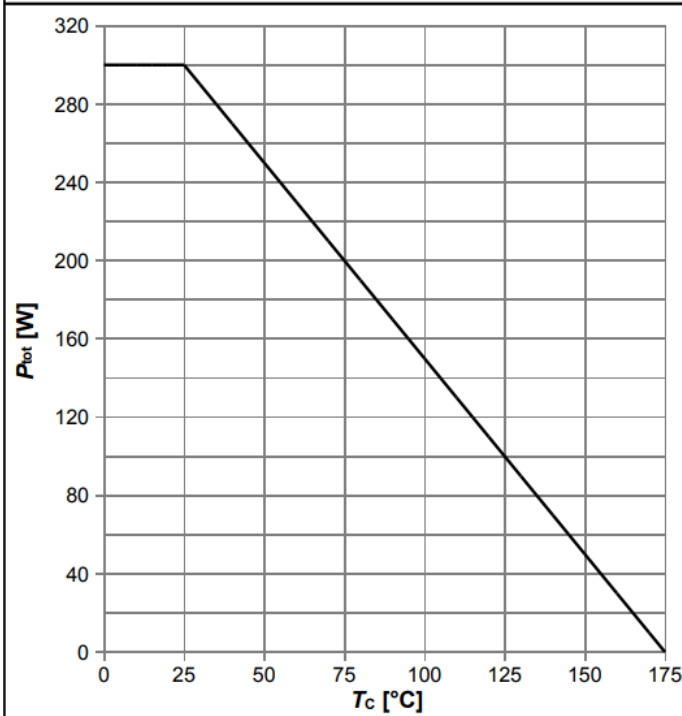
Diagram 1: Power dissipation
