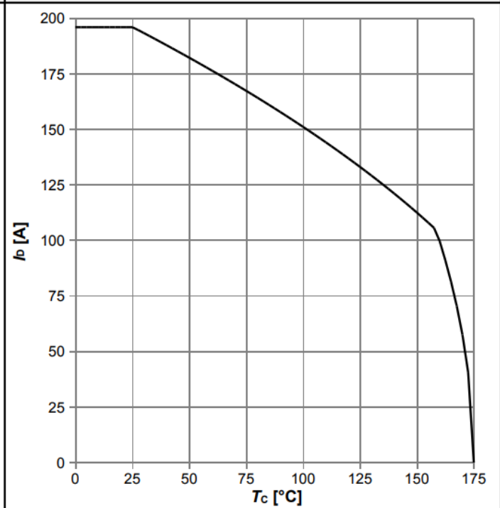
Diagram 2: Drain current
