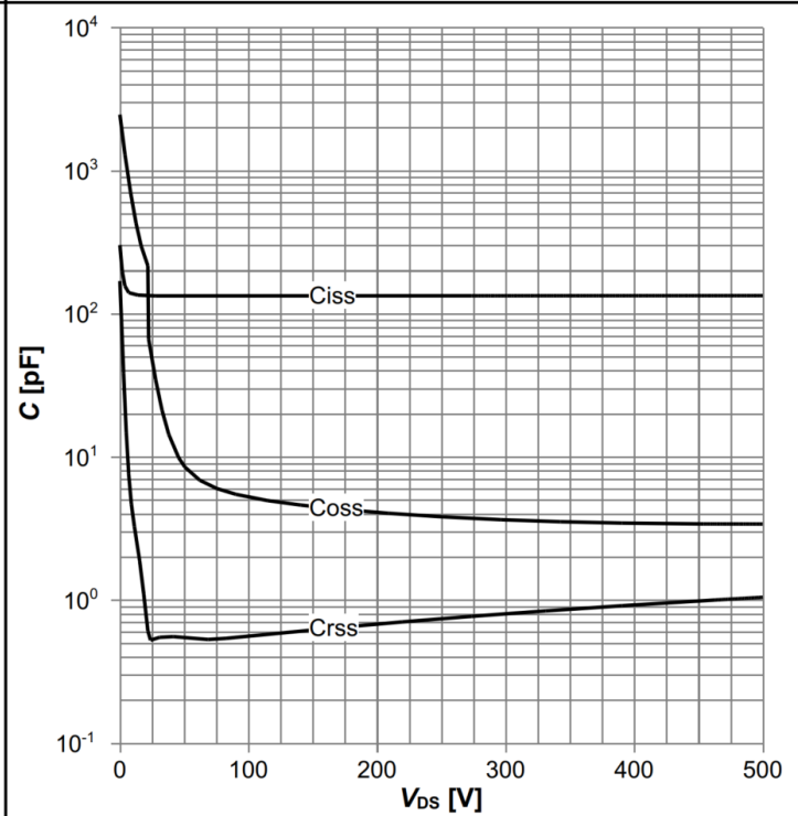
Diagram 14: Typ. capacitances
