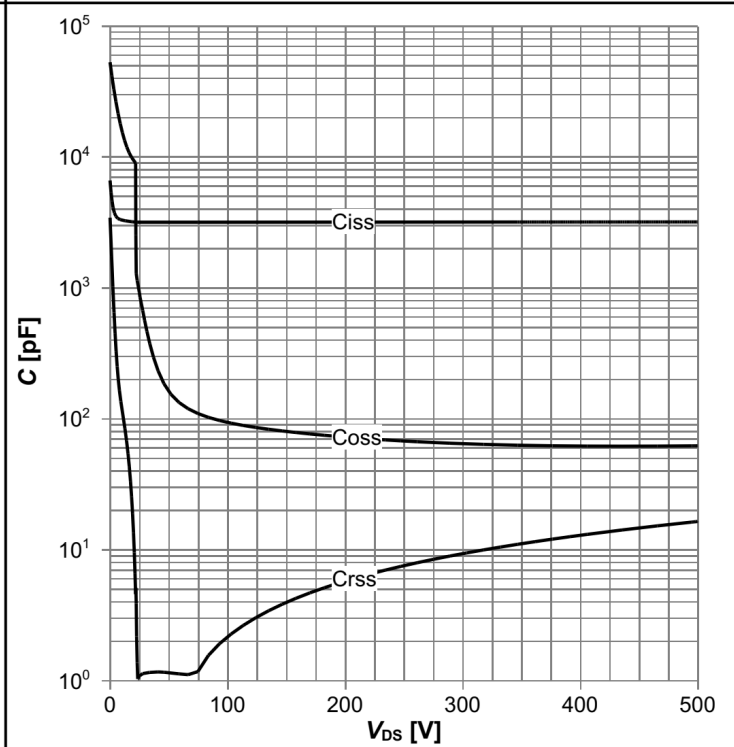
Diagram 14: Typ. capacitances
