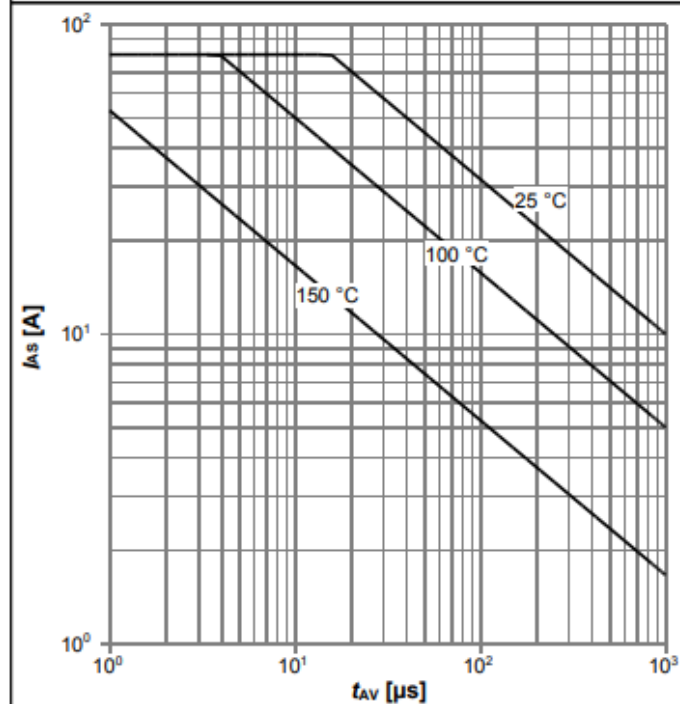
Diagram 13: Avalanche characteristics
