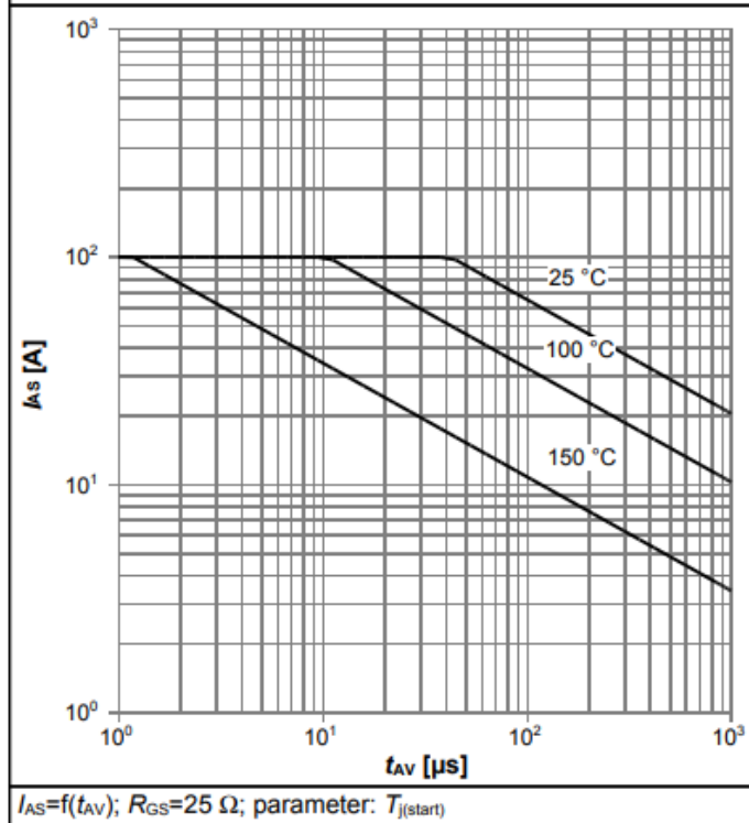
Diagram 13: Avalanche characteristics
