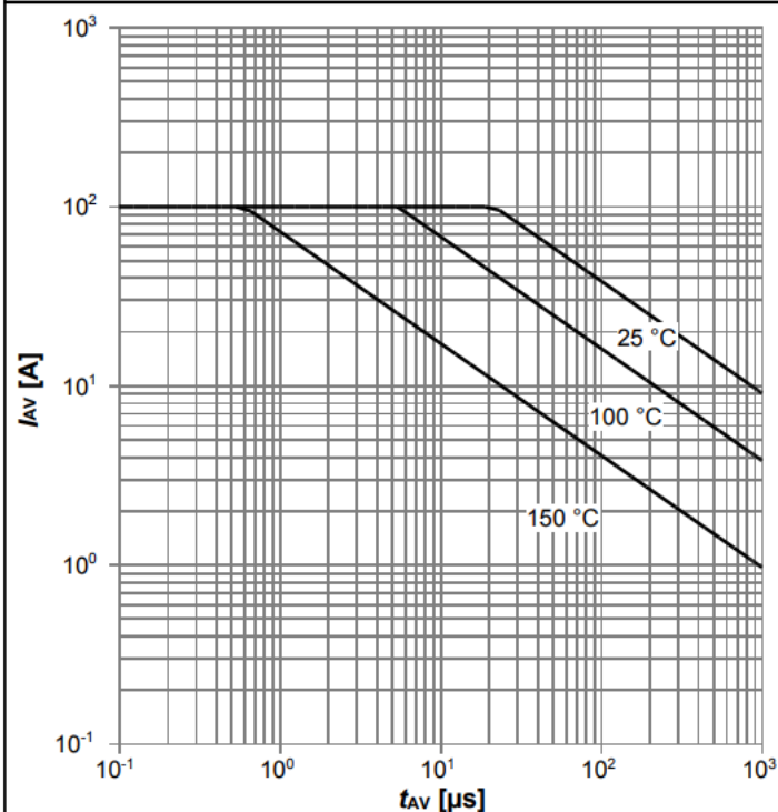
Diagram 13: Avalanche characteristics
