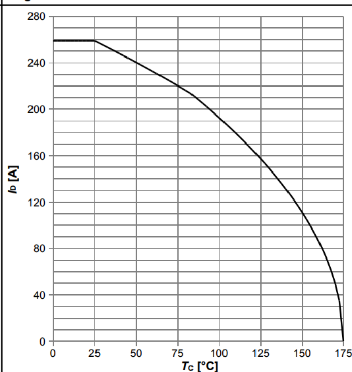
Diagram 2: Drain current
