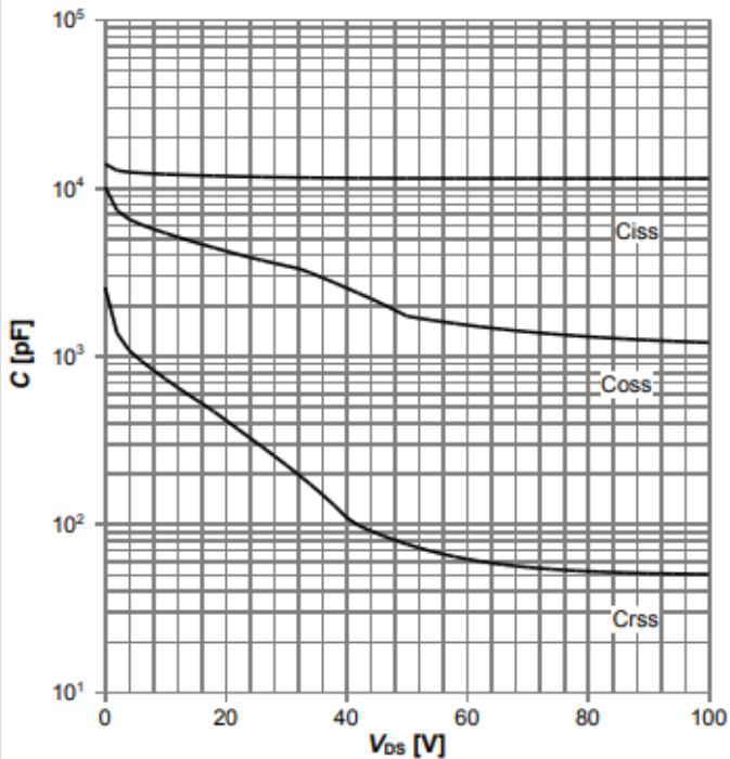
Diagram 11: Typ. capacitances
