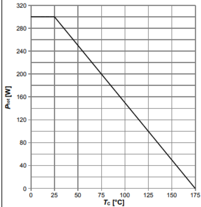
Diagram 1: Power dissipation
