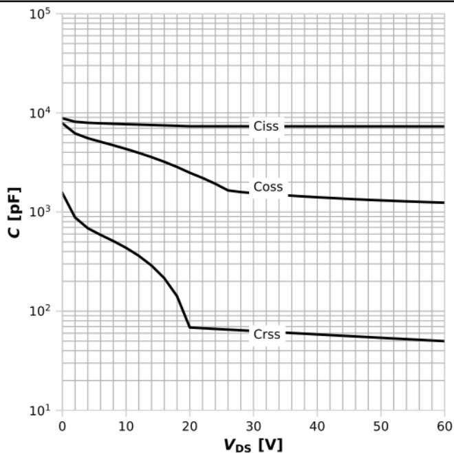
Diagram 11: Typ. capacitances
