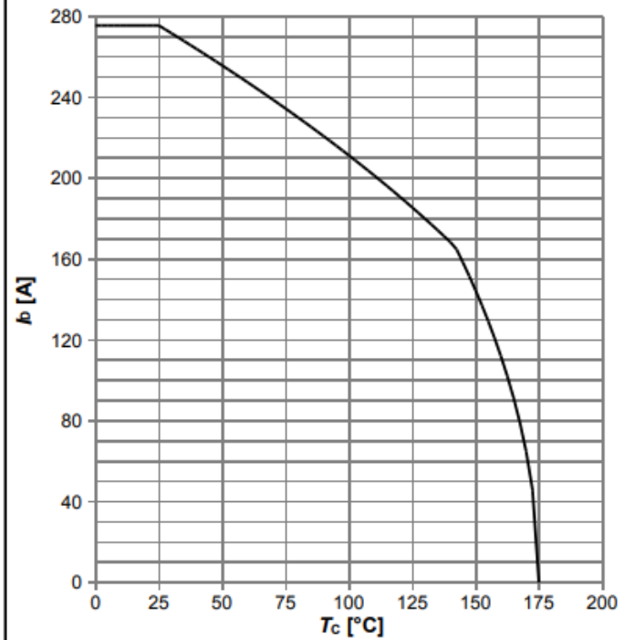
Diagram 2: Drain current
