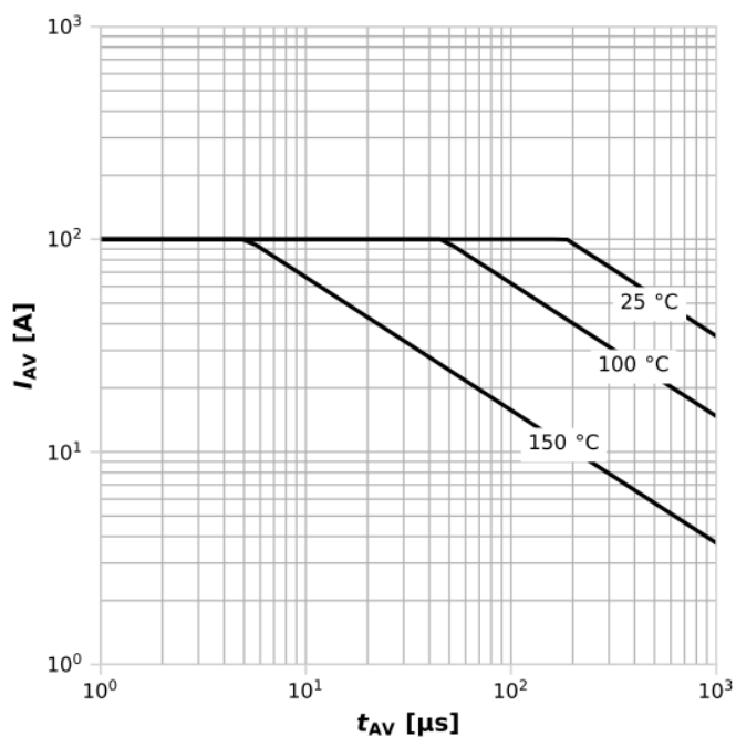
Diagram 13: Avalanche characteristics
