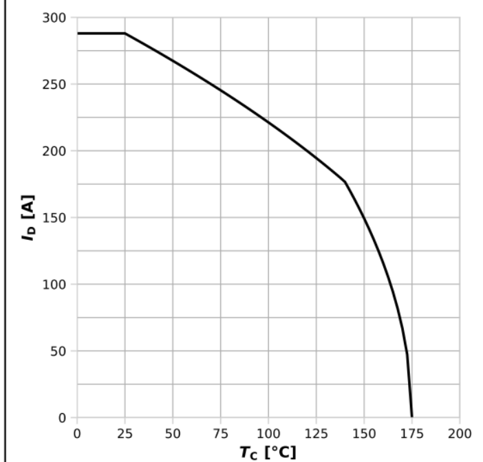
Diagram 2: Drain current
