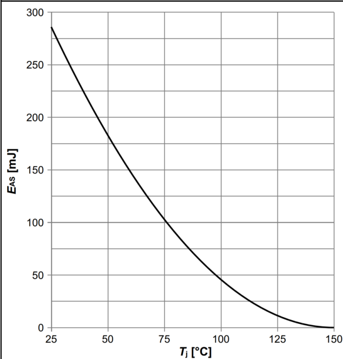
Diagram 13: Avalanche energy
