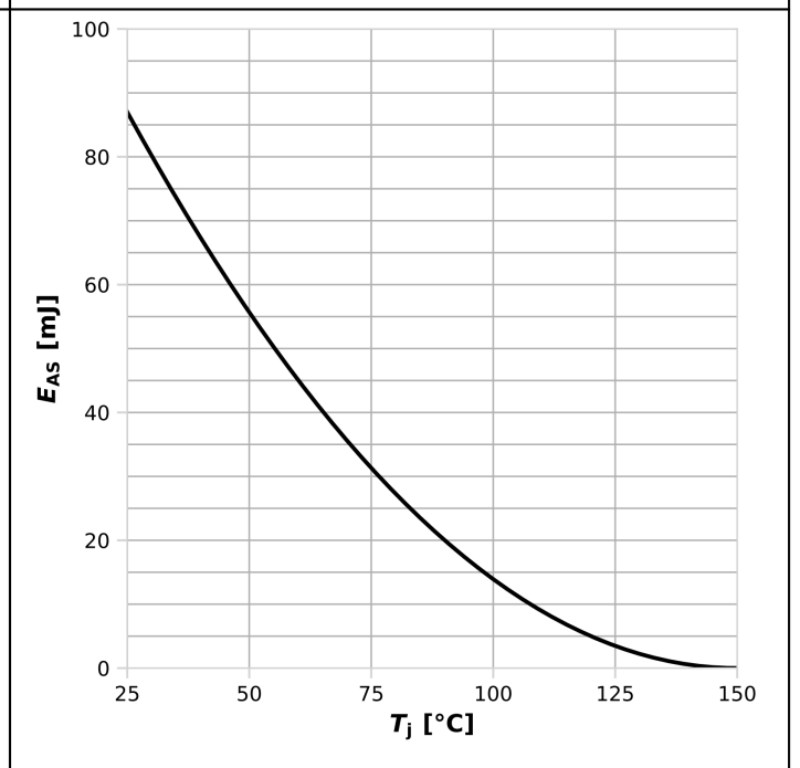
Diagram 12: Avalanche energy
