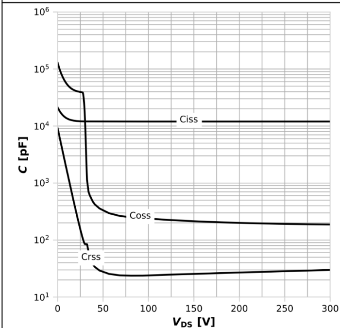
Diagram 15: Typ. capacitances
