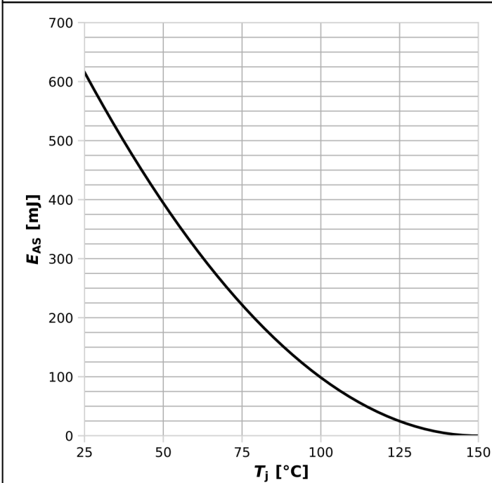
Diagram 13: Avalanche energy
