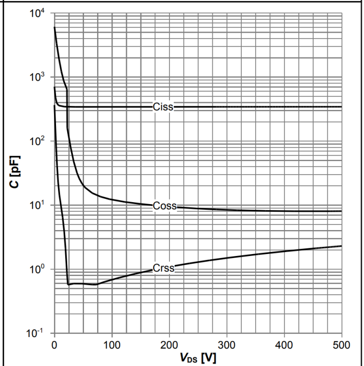
Diagram 14: Typ. capacitances
