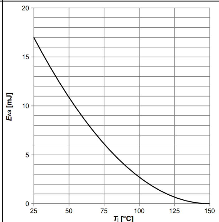
Diagram 12: Avalanche energy
