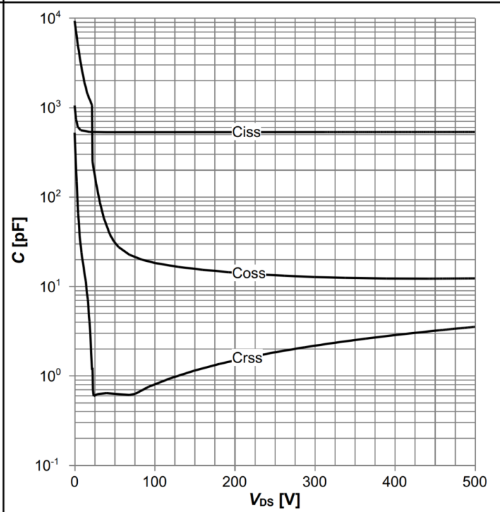
Diagram 14: Typ. capacitances
