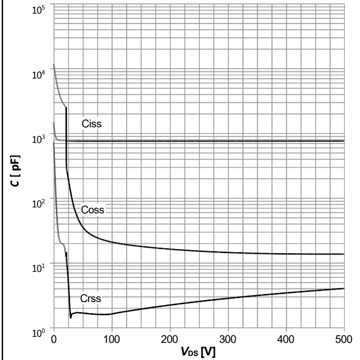
Diagram 14: Typ. capacitances
