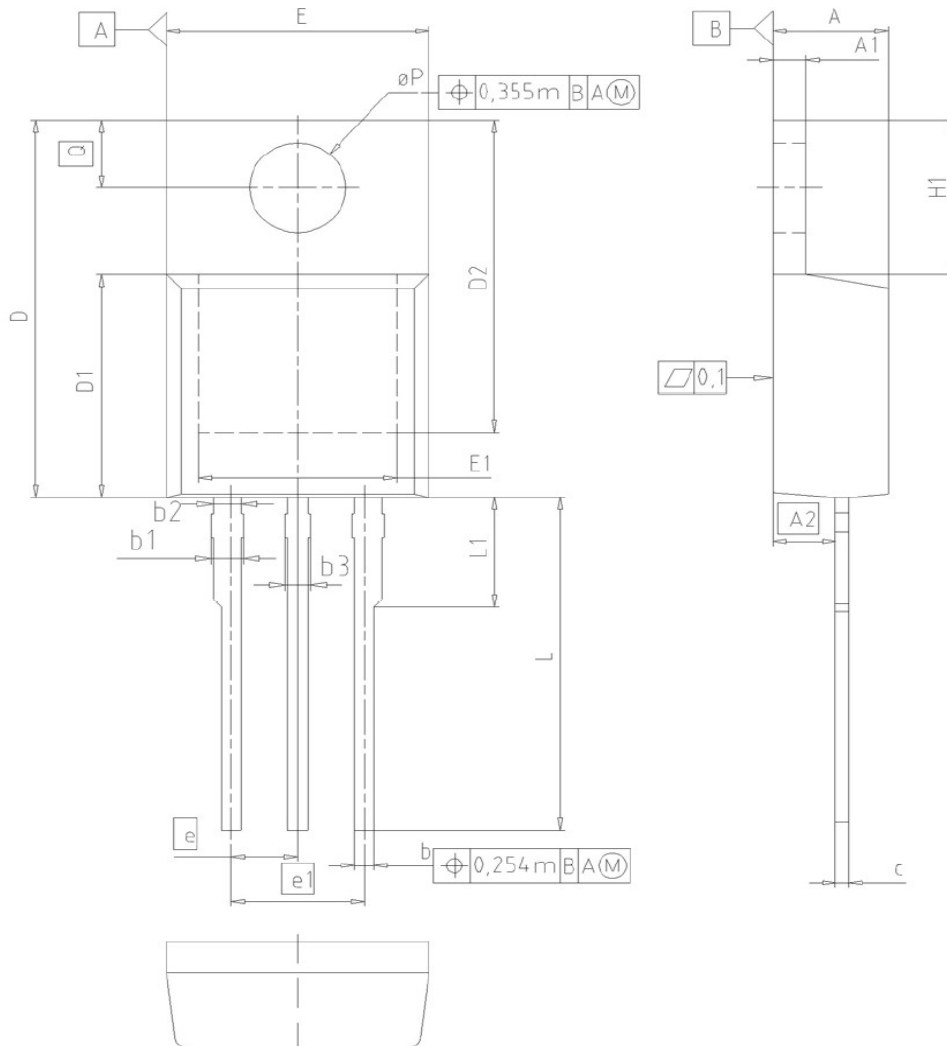
PG-T0220-3: 外形图
