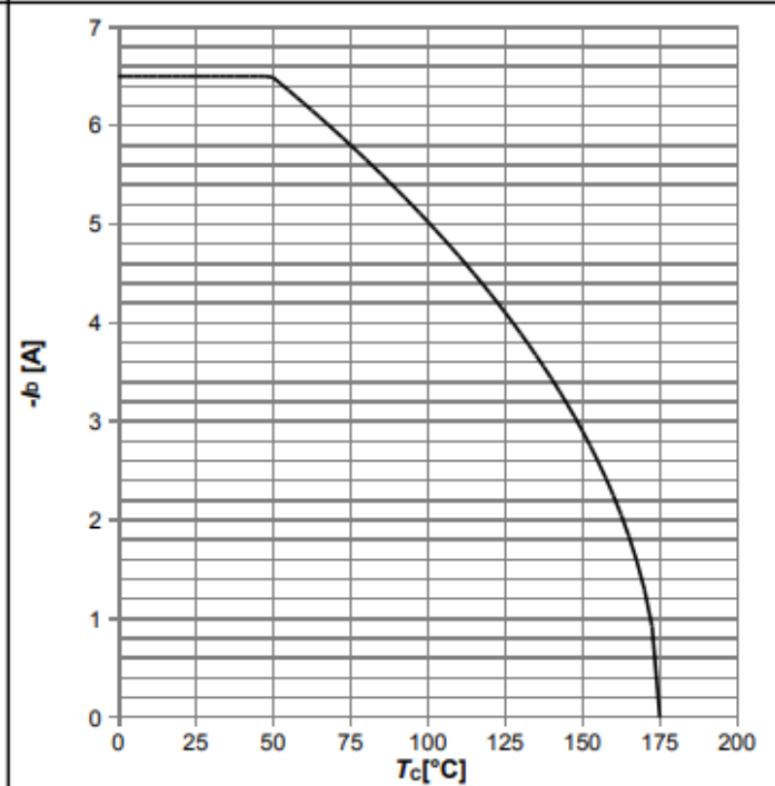
Diagram 2: Drain current
