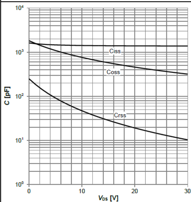
Diagram 11: Typ. capacitances
