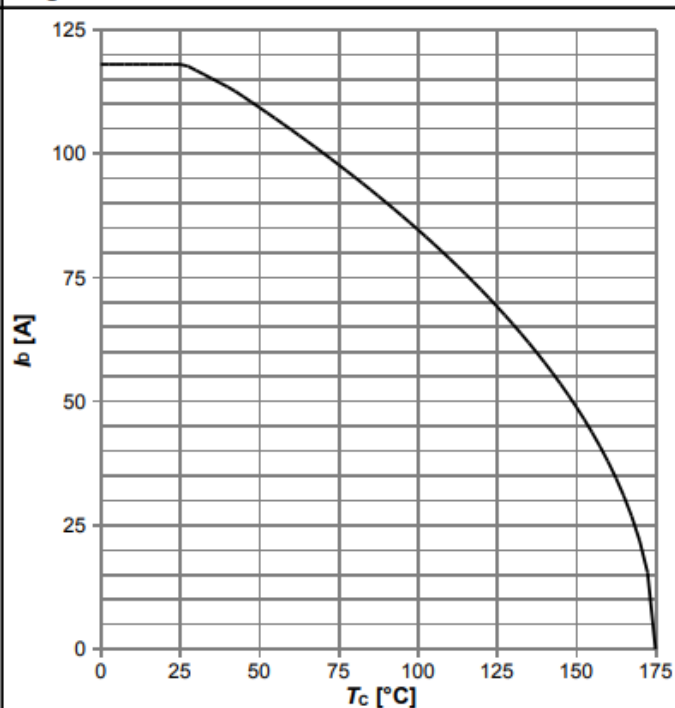
Diagram 2: Drain current
