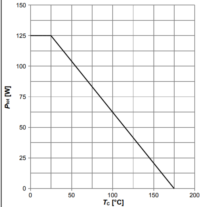
Diagram 1: Power dissipation
