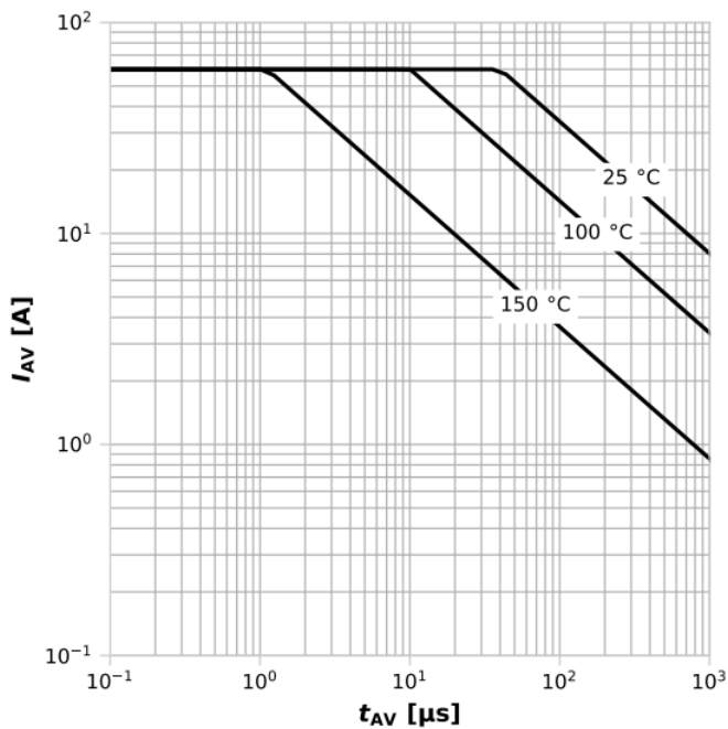
Diagram 13: Avalanche characteristics
