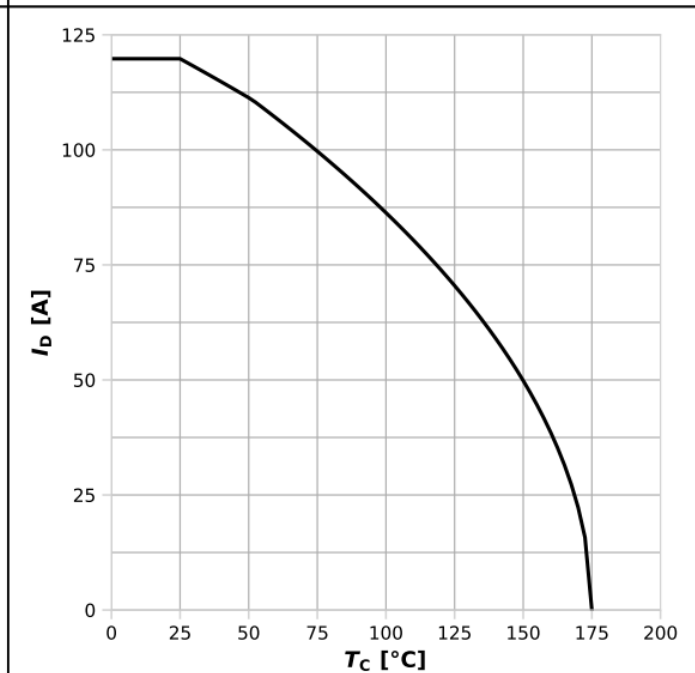
Diagram 2: Drain current
