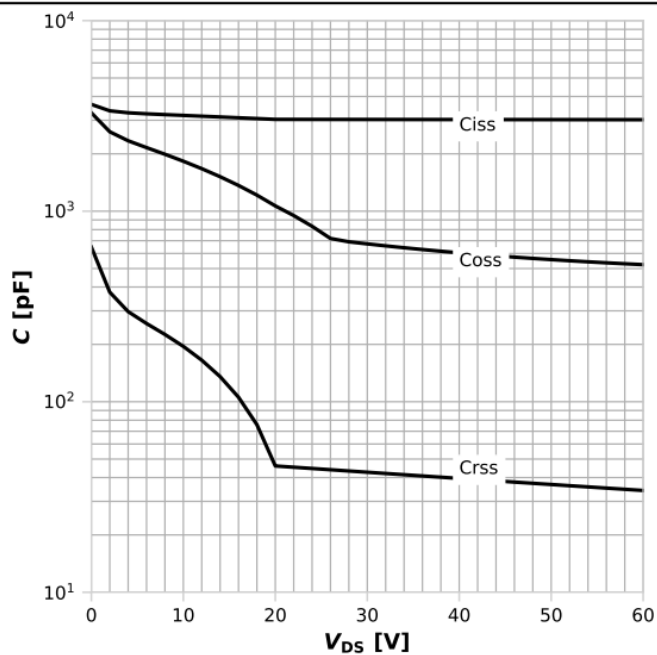
Diagram 11: Typ. capacitances
