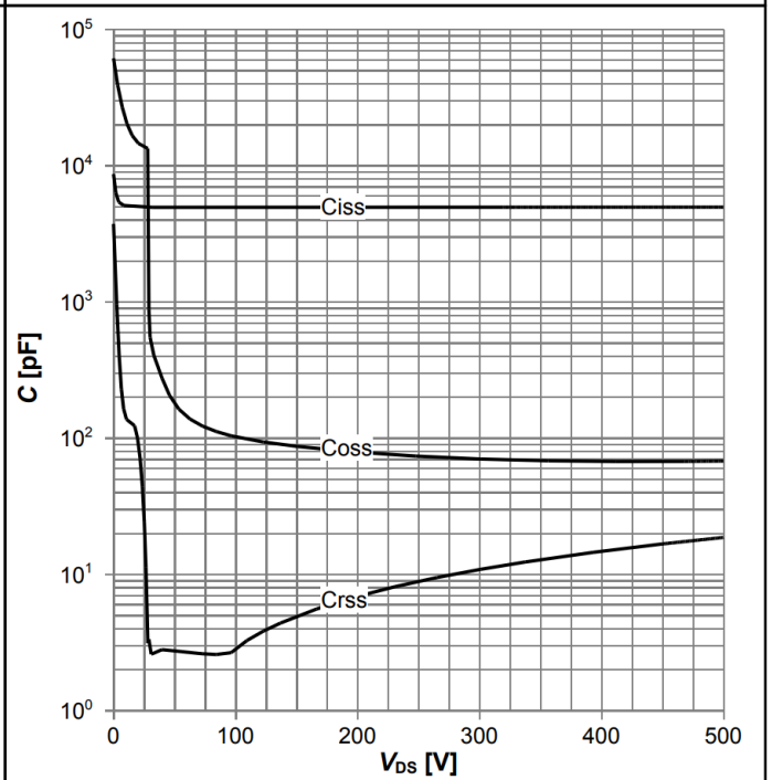
Diagram 14: Typ. capacitances
