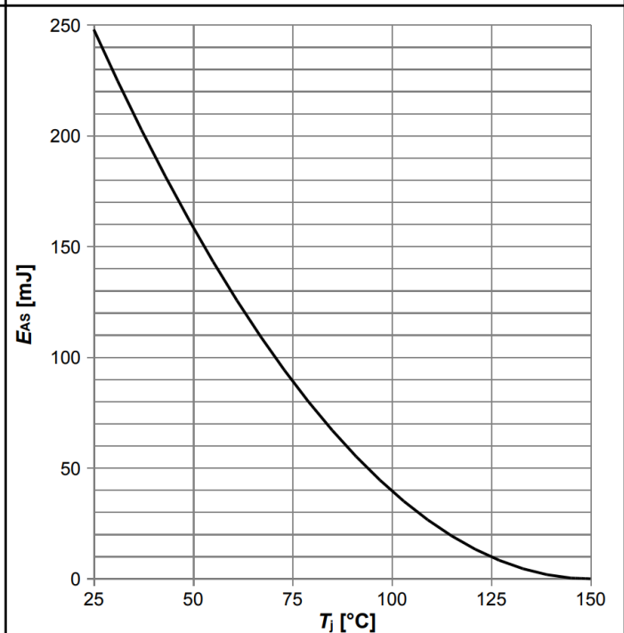
Diagram 12: Avalanche energy
