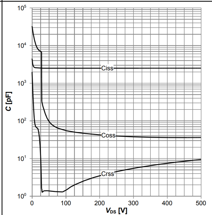
Diagram 14: Typ. capacitances
