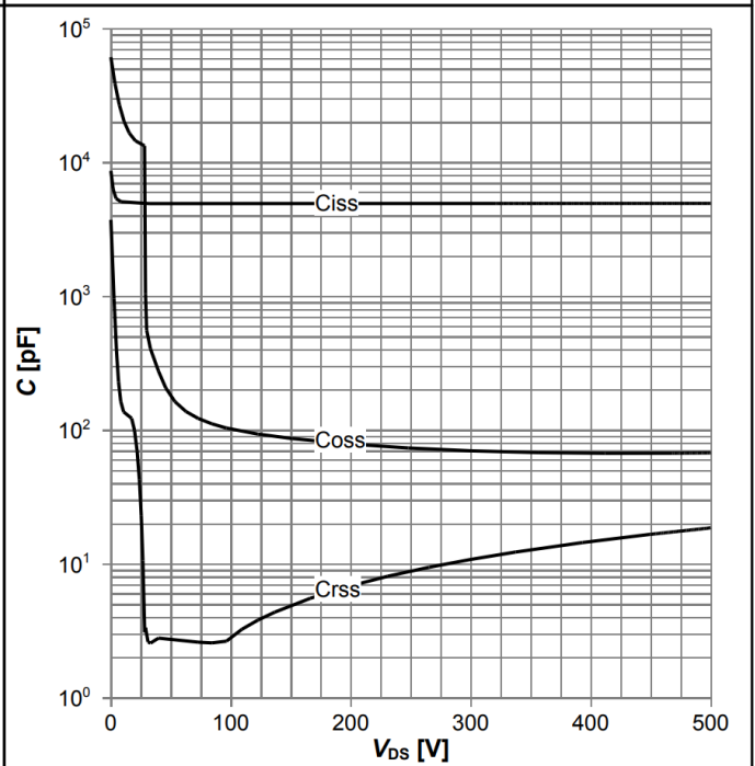
Diagram 14: Typ. capacitances
