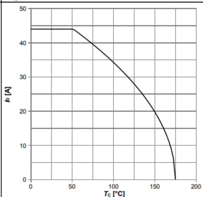
Diagram 2: Drain current
