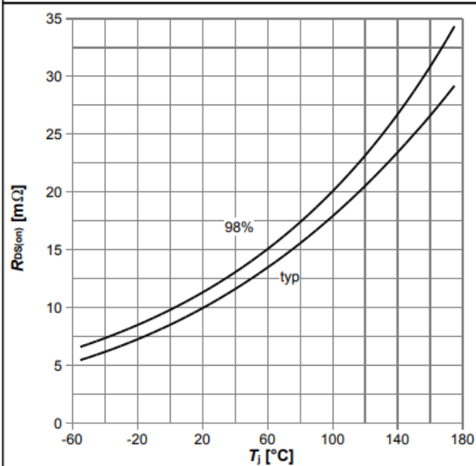
Diagram 9: Drain-source on-state resistance
