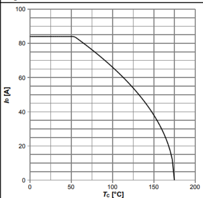
Diagram 2: Drain current
