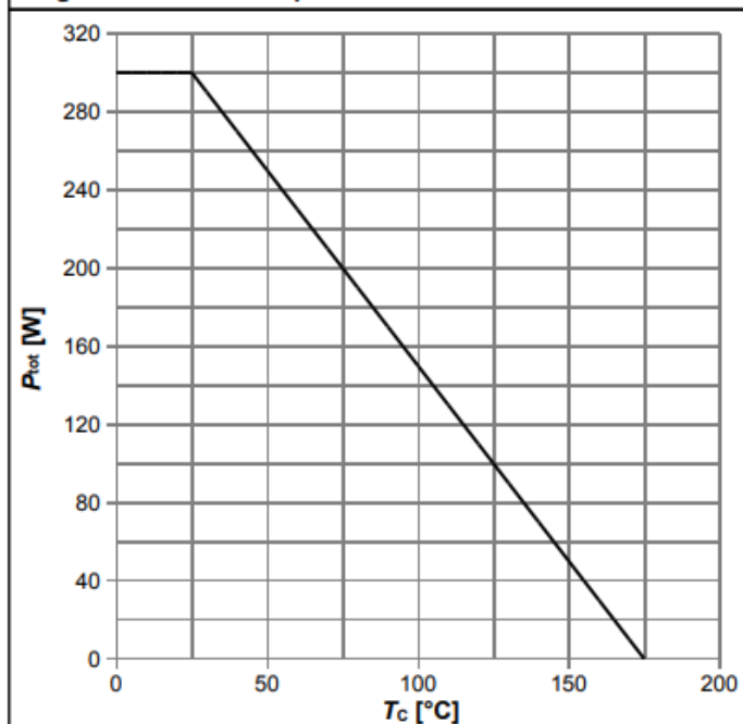
Diagram 1: Power dissipation
