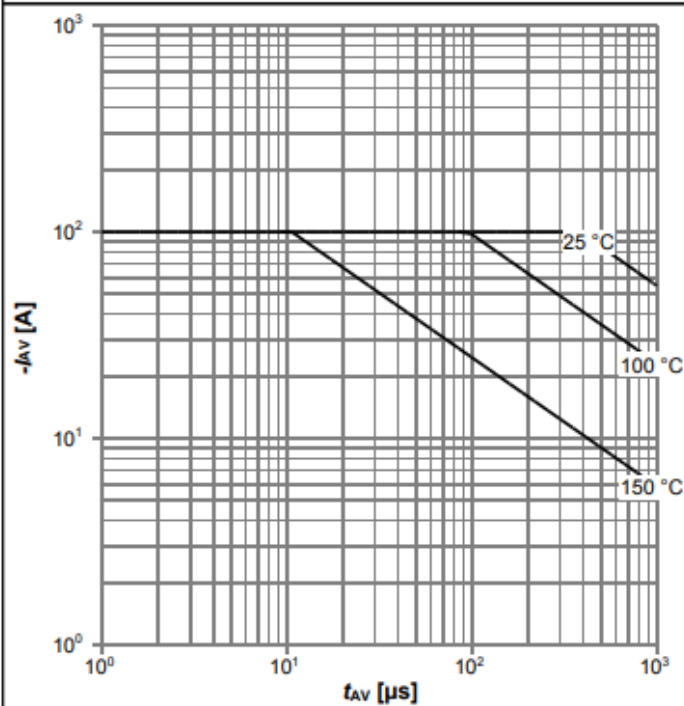
Diagram 13: Avalanche characteristics
