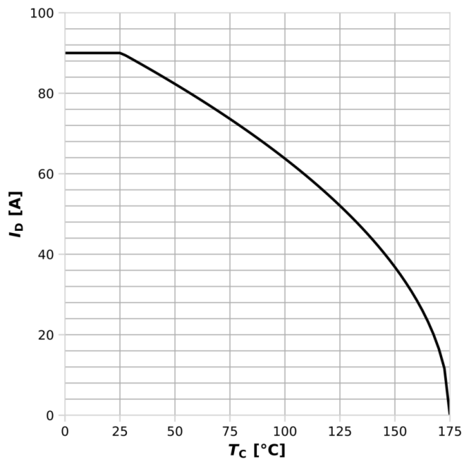
Diagram 2: Drain current
