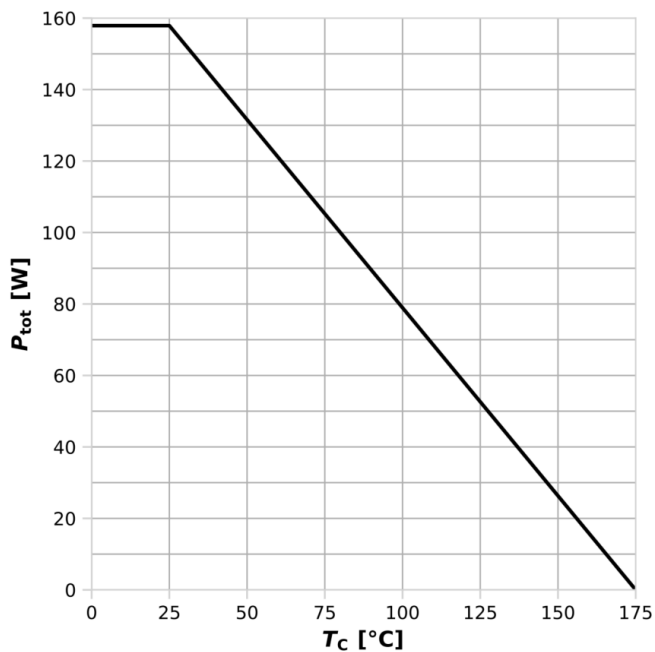
Diagram 1: Power dissipation
