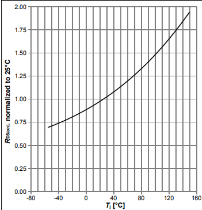
Diagram 9: Normalized drain-source on-state resistance
