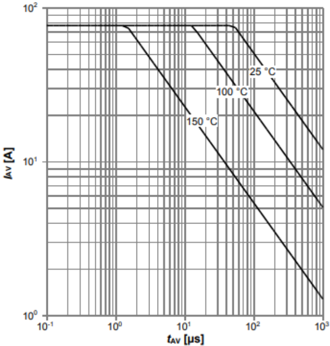
Diagram 13: Avalanche characteristics
