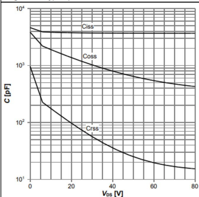
Diagram 11: Typ. capacitances
