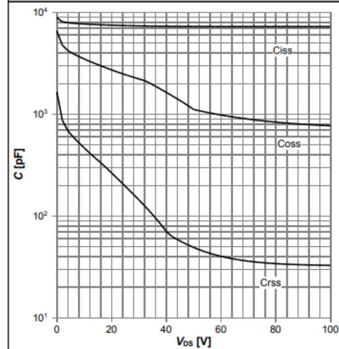
Diagram 11: Typ. capacitances
