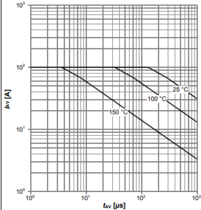
Diagram 13: Avalanche characteristics
