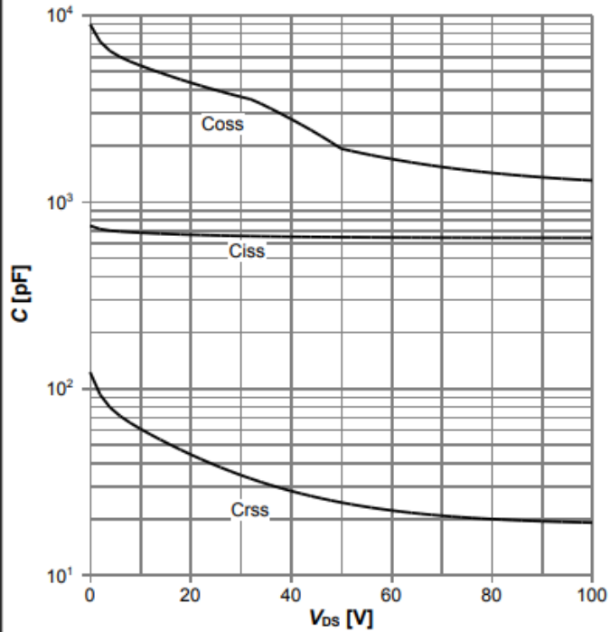
Diagram 11: Typ. capacitances
